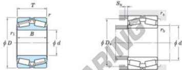
Double-row tapered roller bearings TDI type Koyo
