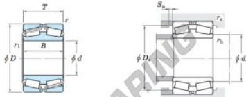
Double-row tapered roller bearings TDI type Koyo
