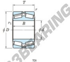
Boundary dimensions
