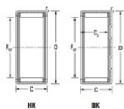
Boundary dimensions
