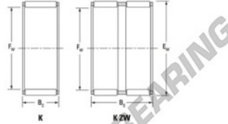
Needle roller and cage assemblies
