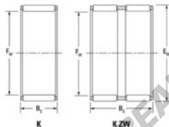
Basic rated roller and cage assemblies
