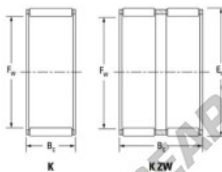
Boundary dimensions
