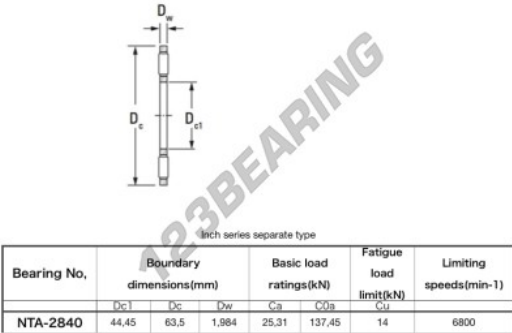
Boundary dimensions
