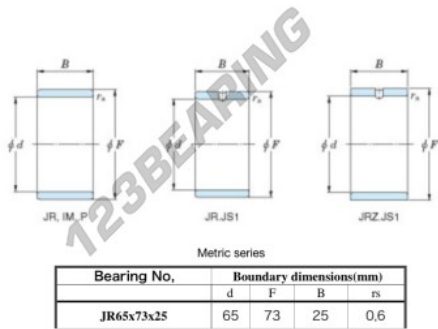
Boundary dimensions
